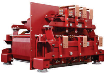
■ Auxiliary Transformer
